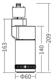
3-pin track adaptor
